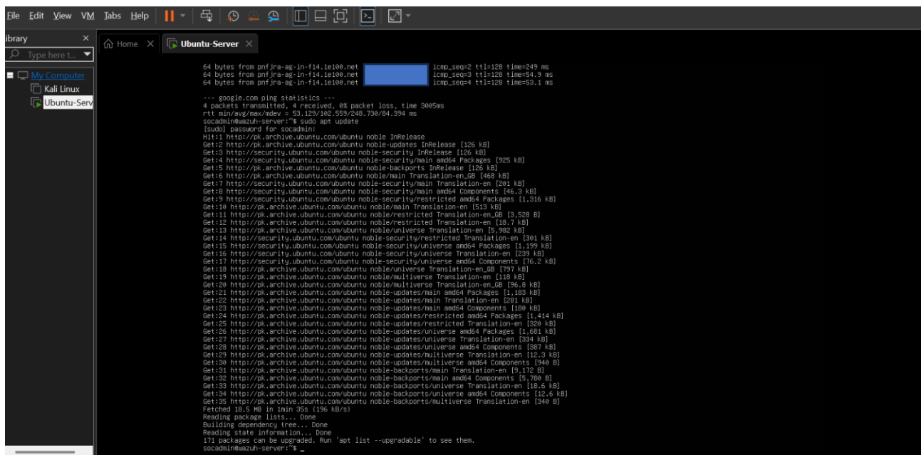
Figure 4.2 System Update
