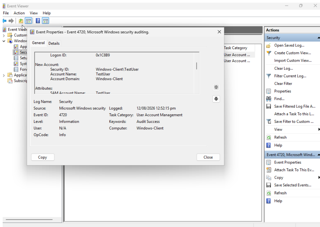
Figure 7.2 Window event
