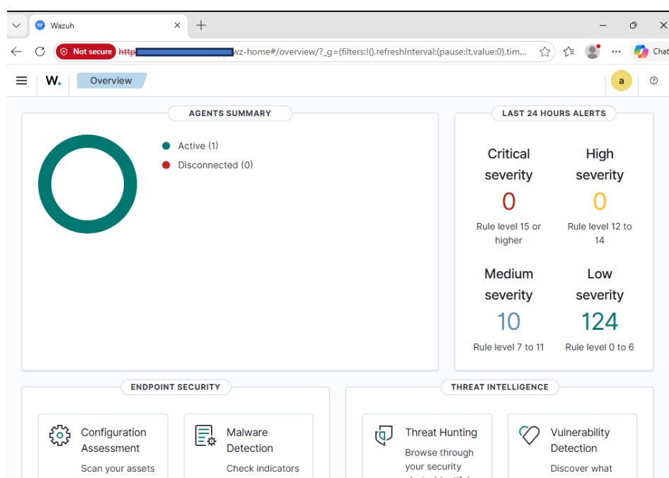
Figure 6.1 Dashboard Overview
