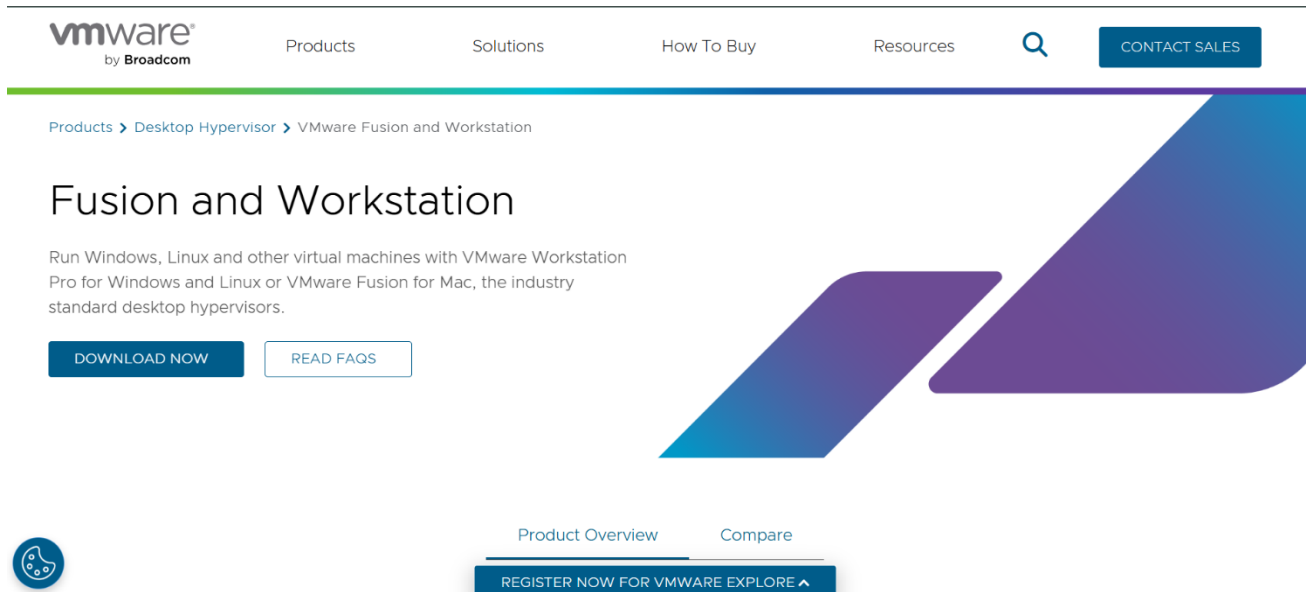
Figure 3.4 VMware Installation
