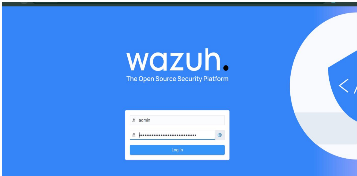
Figure 4.10 Login page
