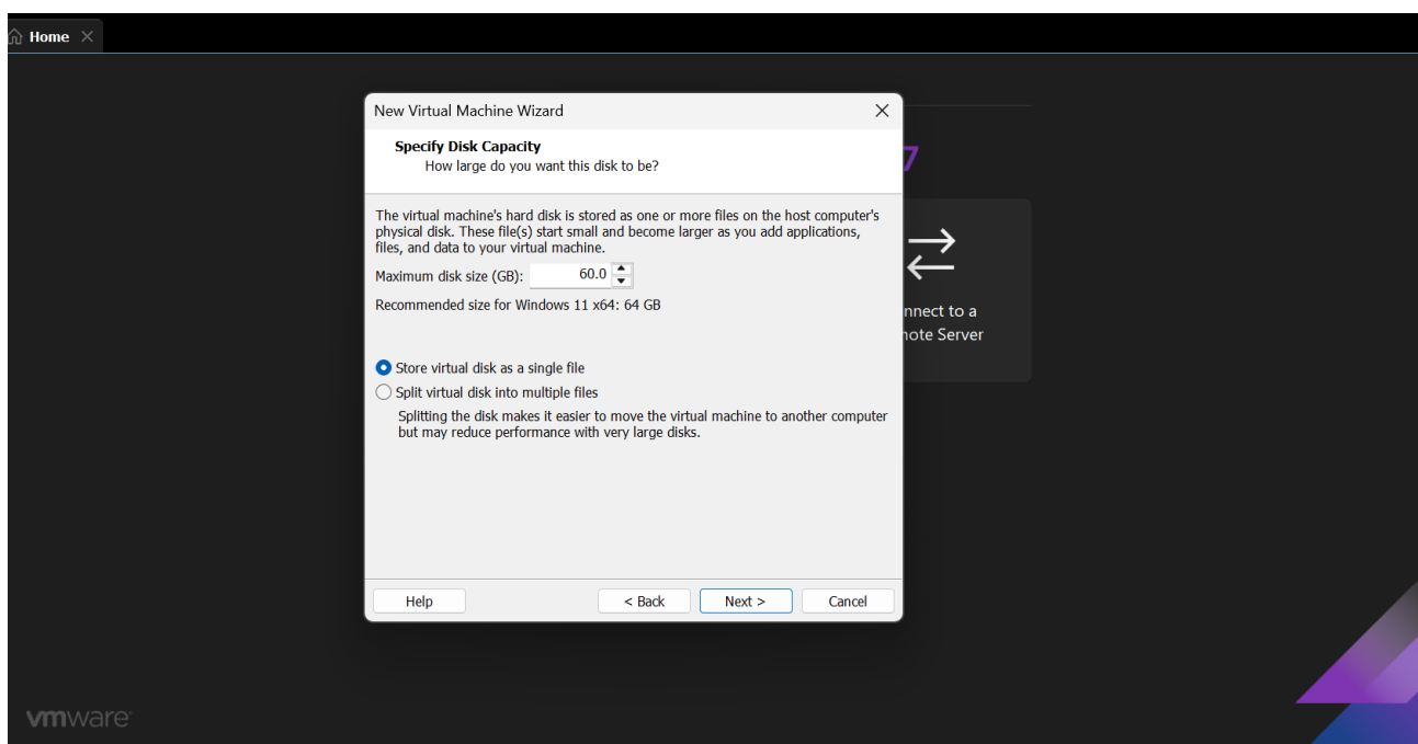
Figure 3.10 Disk capacity
