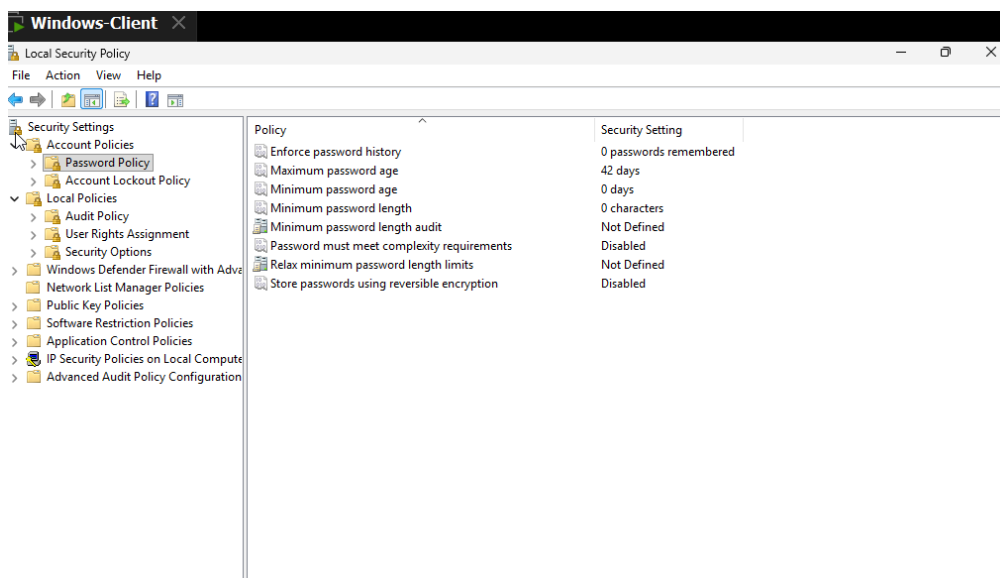
Figure 5.5 Password Policy
