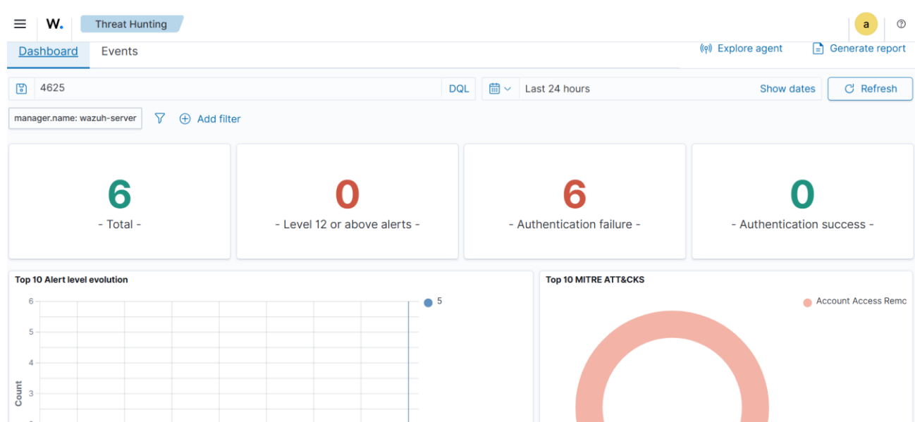
Figure 8.5 Alert generated
