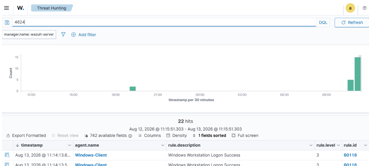
Figure 7.16 Wazuh Detection
