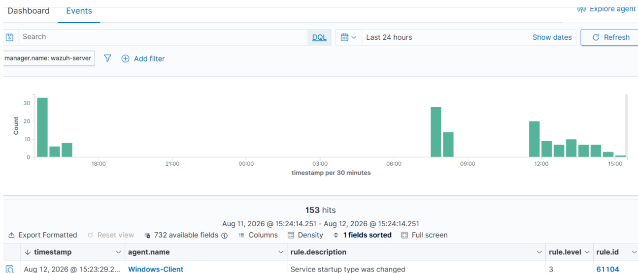
Figure 7.14 Wazuh Detection
