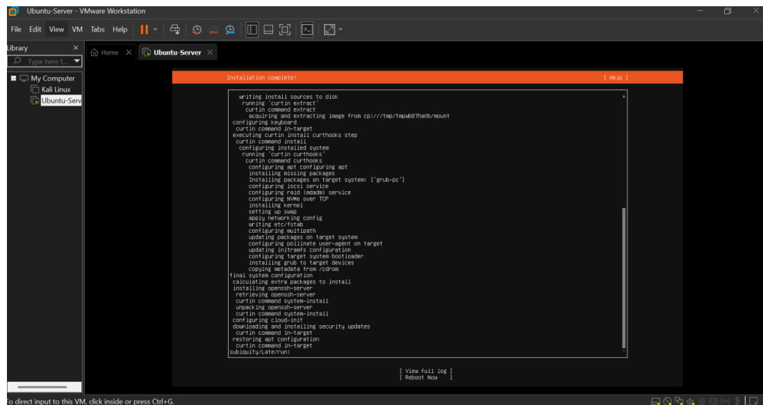
Figure 3.16 Ubuntu Installation
