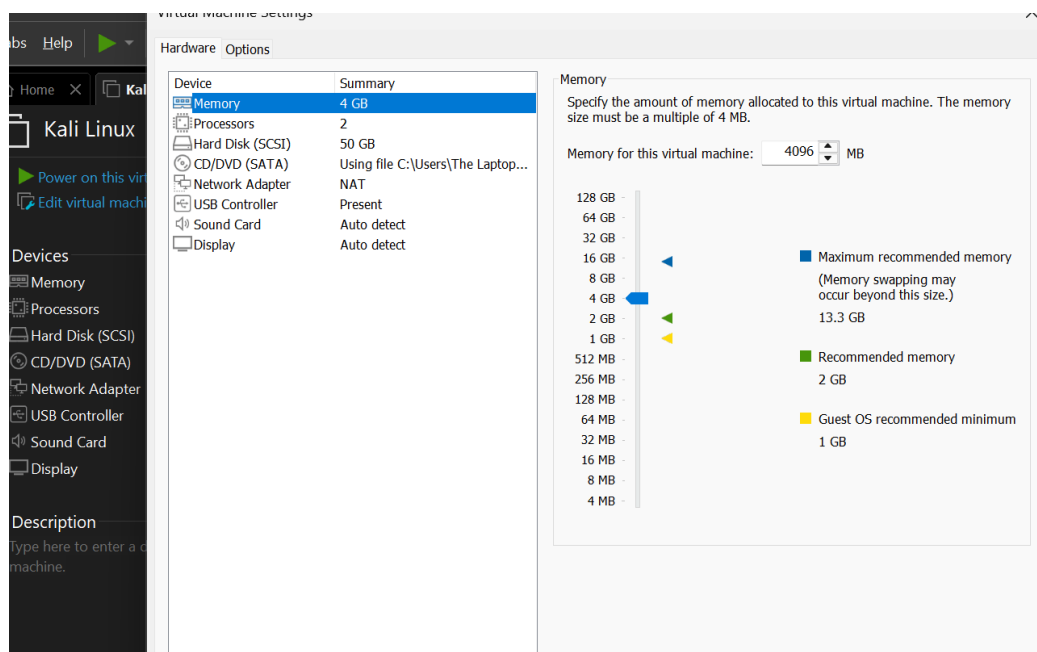
Figure 3.7 Hardware settings
