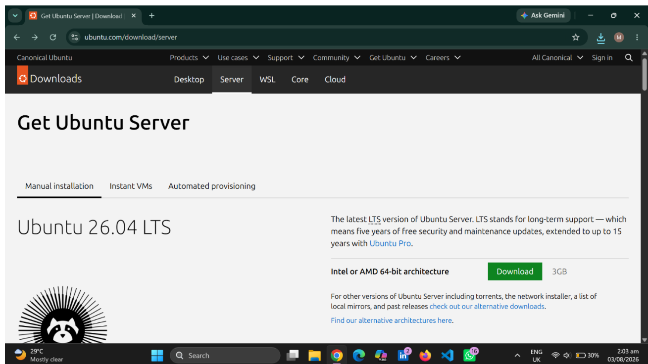
Figure 3.17 Ubuntu version
