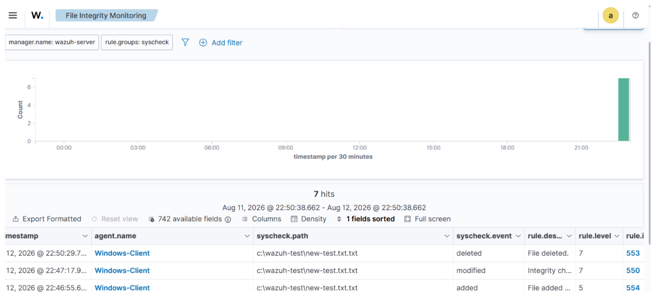
Figure 7.10 Wazuh Alert
