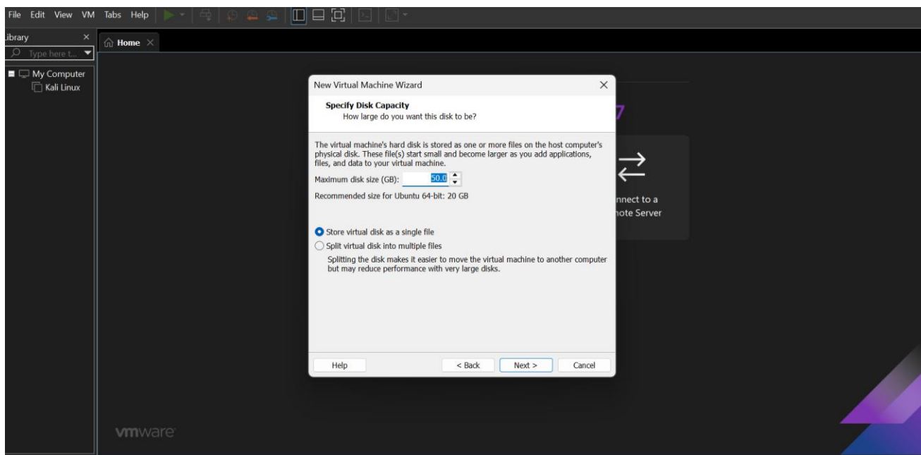
Figure 3.15 Disk Capacity
