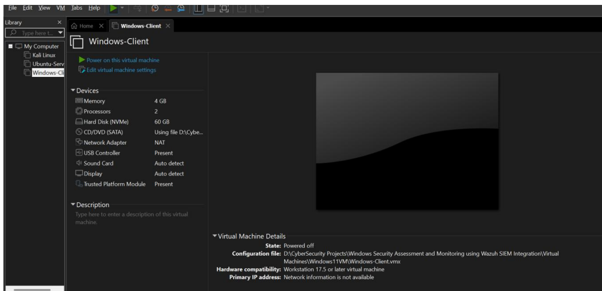
Figure 3.8 VM created
