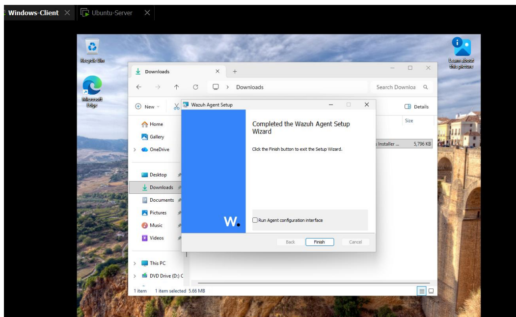
Figure 4.13 Agent Installation
