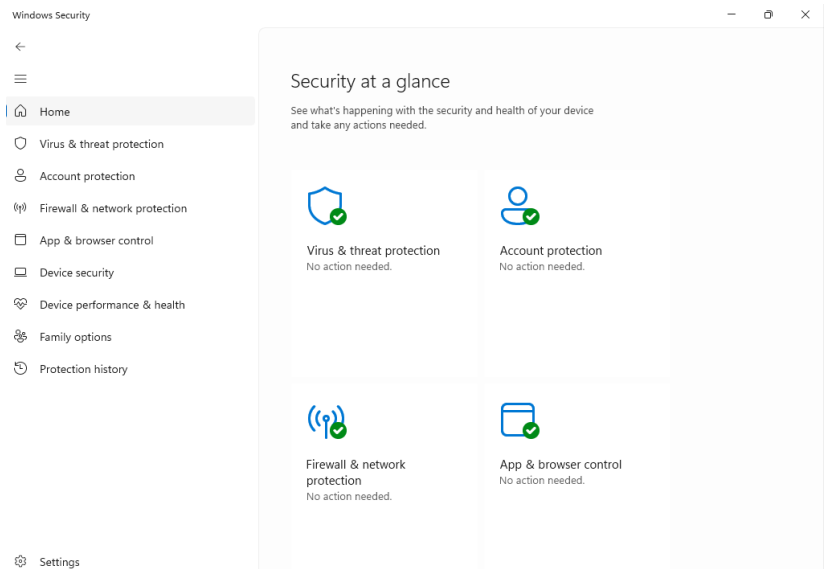
Figure 5.4 After assessment
