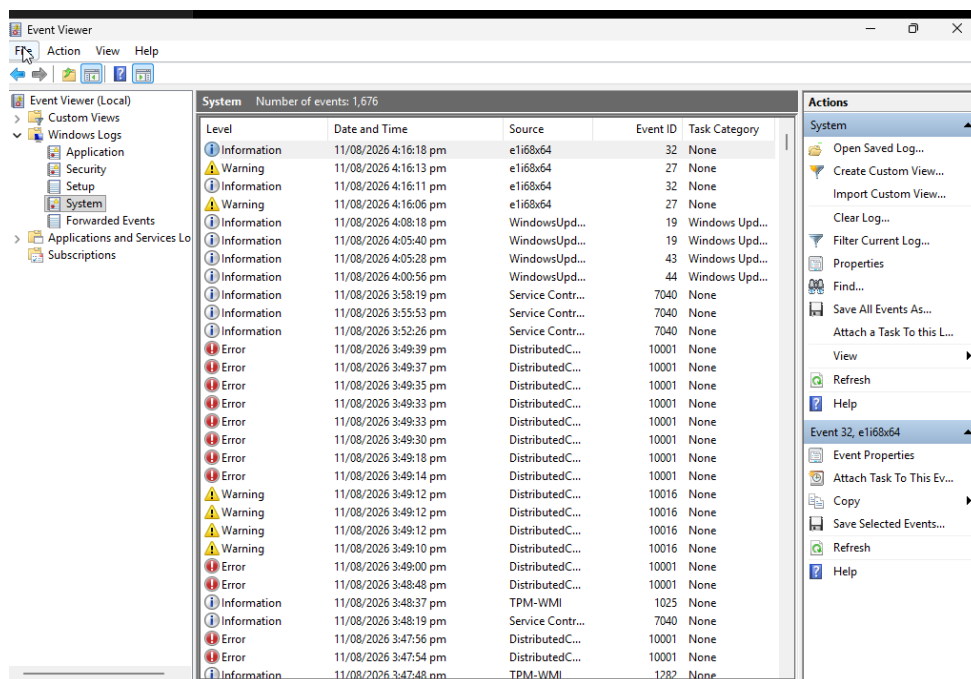
Figure 5.15 System Logs
