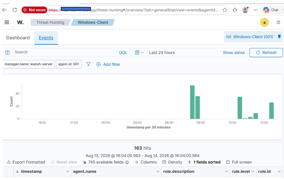
Figure 6.3 Event Section
