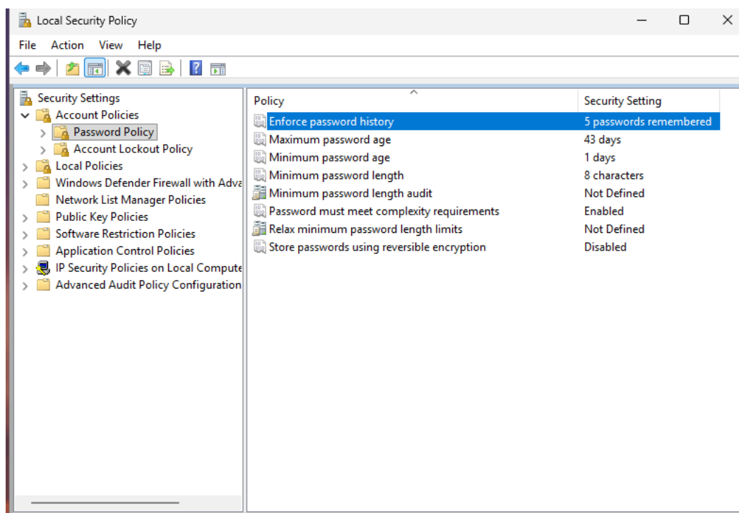
Figure 5.6 After Assessment
