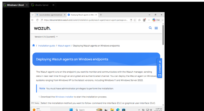
Figure 4.12 Agent downloaded
