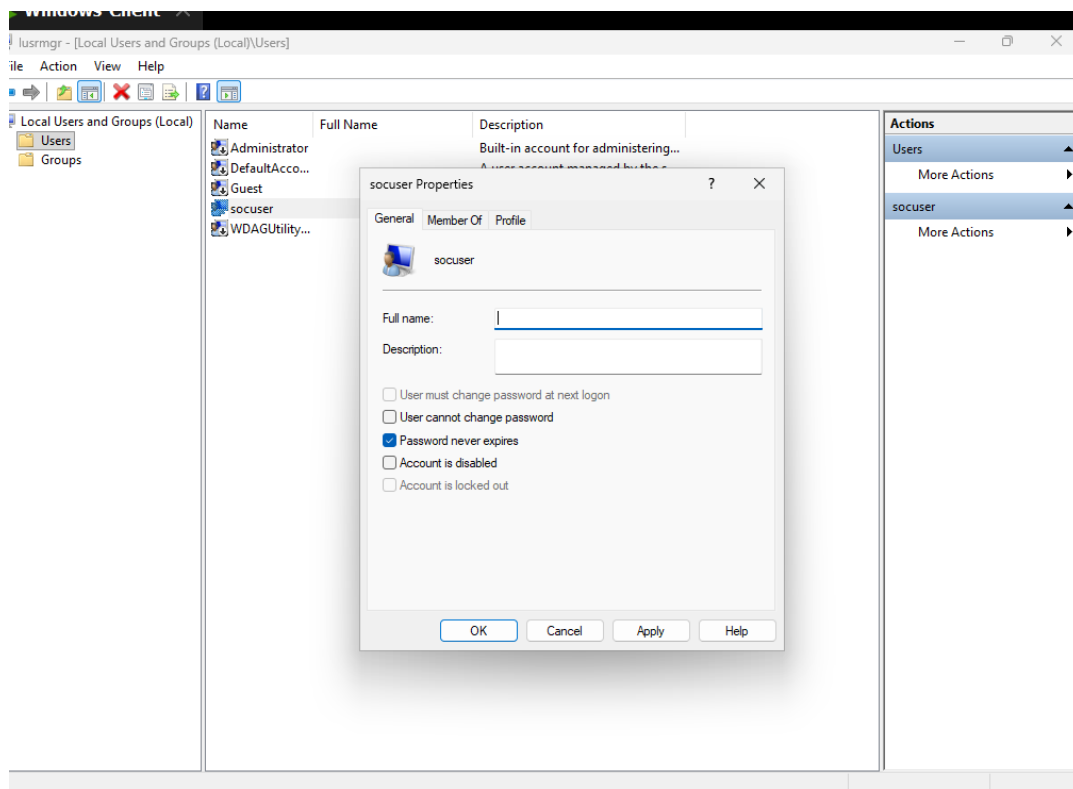
Figure 5.8 User Account
