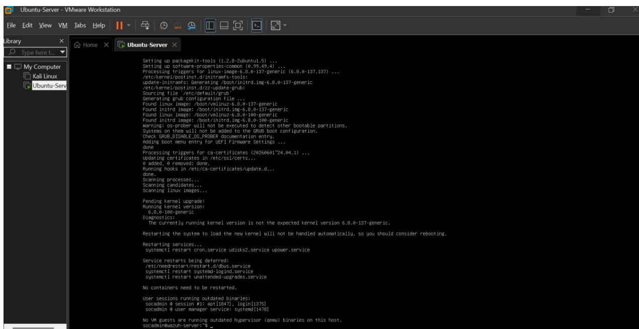
Figure 4.3 System upgraded
