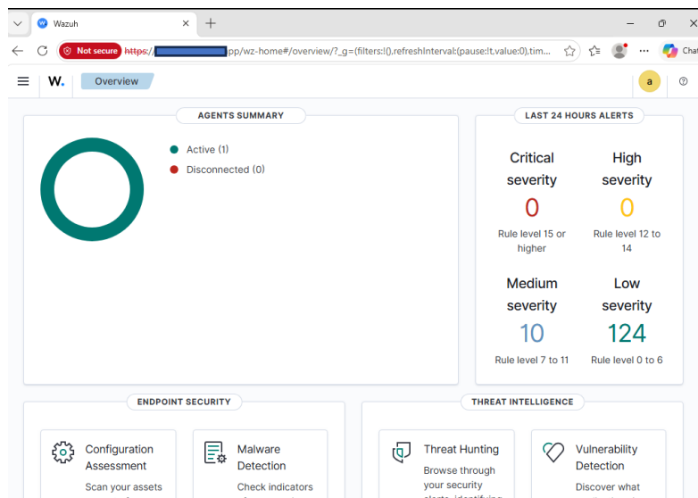
Figure 4.18 Agent Active
