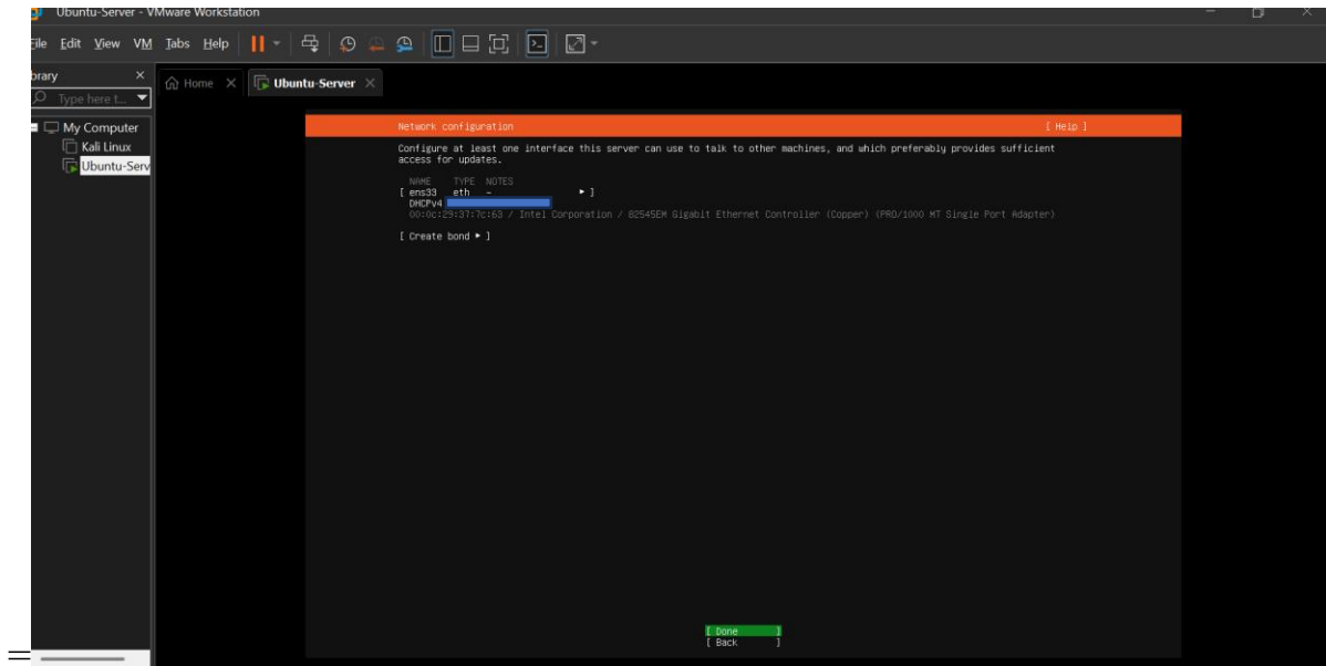
Figure 3.18 Network Configuration
