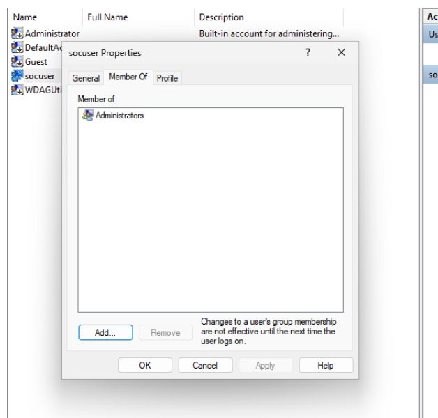
Figure 5.9 After assessment
