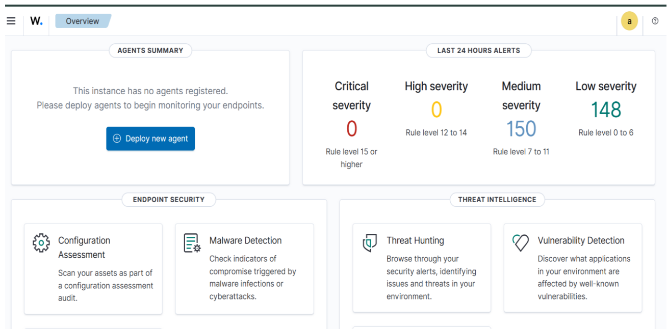
Figure 4.11 Dashboard Homepage
