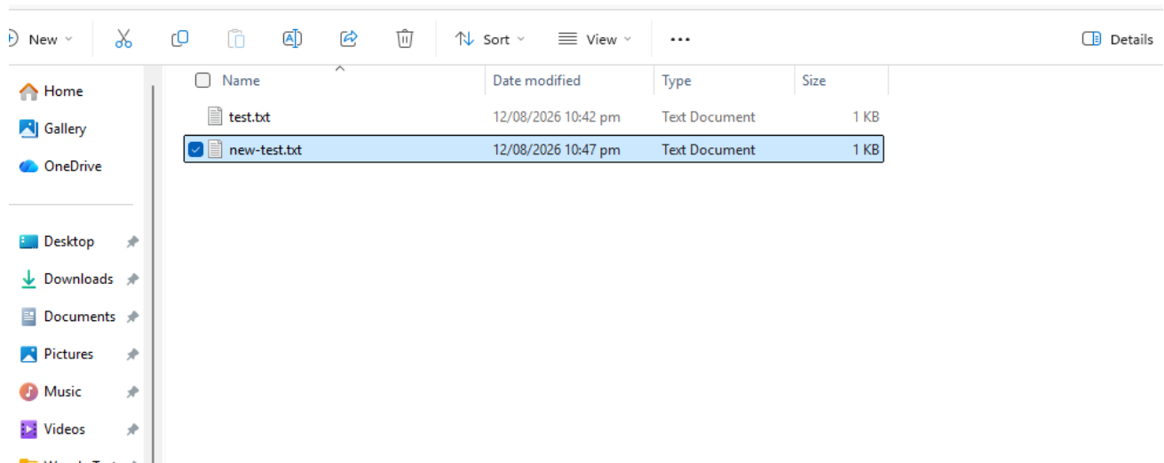
Figure 7.9 File created
