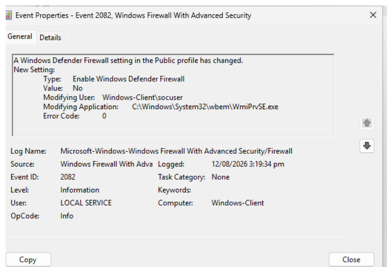
Figure 7.13 windows detected
