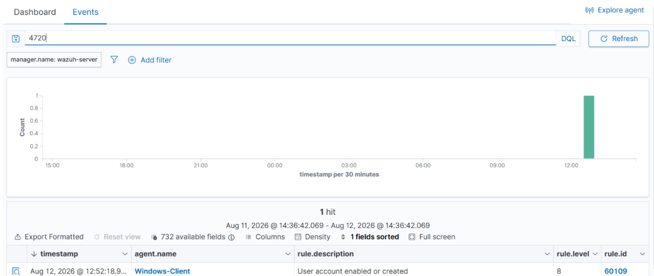
Figure 7.3 wazuh alert
