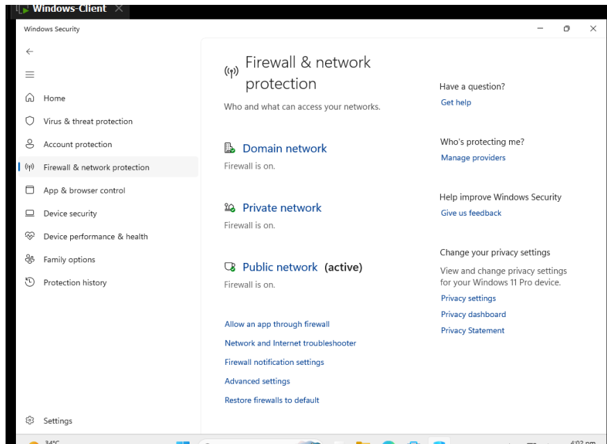
Figure 5.2 Firewall Status
