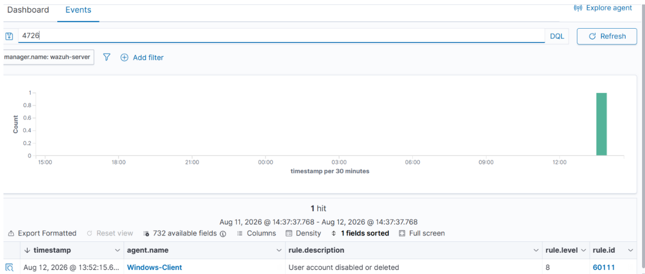
Figure 7.6 Wazuh Deletion Detection
