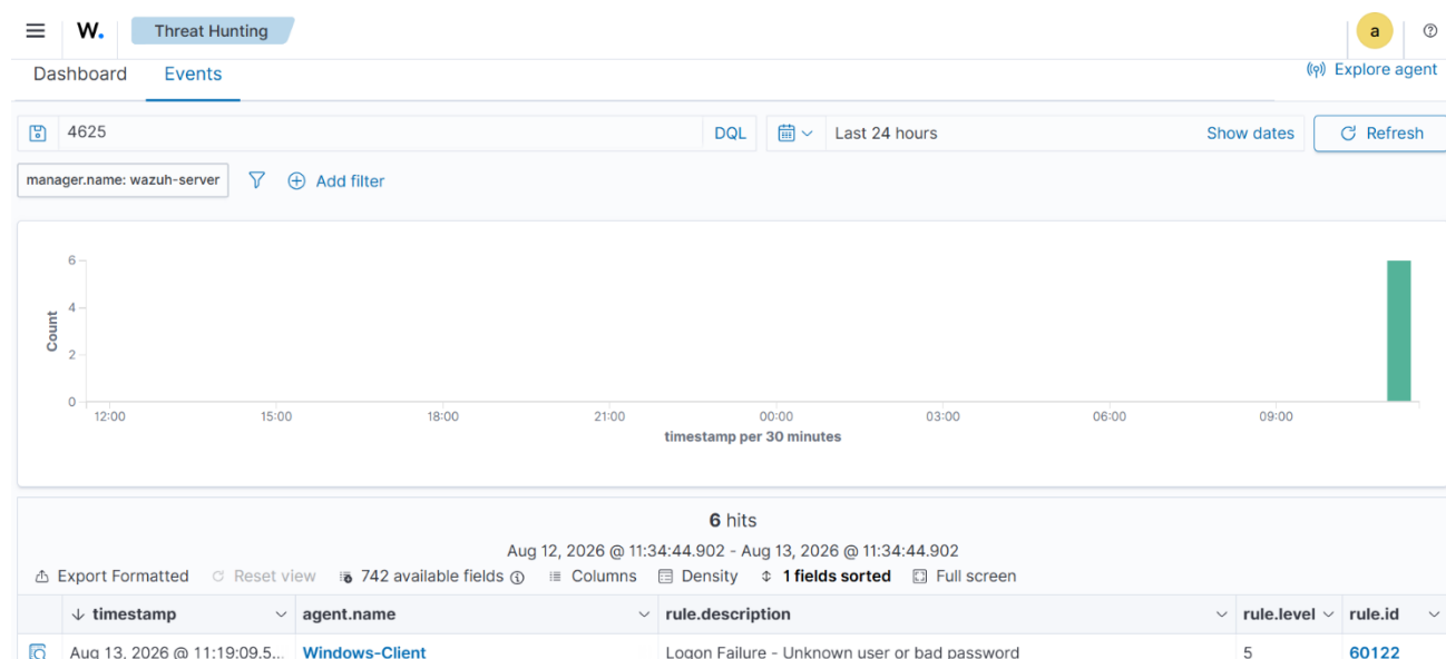
Figure 7.19 Wazuh alert
