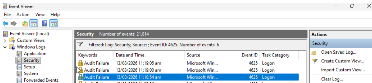
Figure 7.18 login attempts
